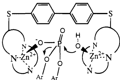
Figure 6. Proposed mechanism for the bifunctional catalysis of the hydrolysis of diester 3 by the bis-zinc complex of ligand 9 . For the cyclization–cleavage of compound 5 and of the dinucleotide UpU, the nucleophile is a coordinated alkoxide ion.
