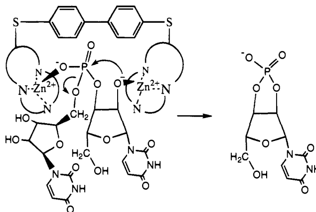
Figure 7. Proposed mechanism for the bifunctional catalysis of the hydrolysis of 3',5'-uridylyridine (UpU) by the bis-zinc complex of ligand 9 . The attack by the coordinated 2' oxide anion may lead to a phosphorane intermediate, with eventual displacement of the 5' oxygen of the second uridine unit.
