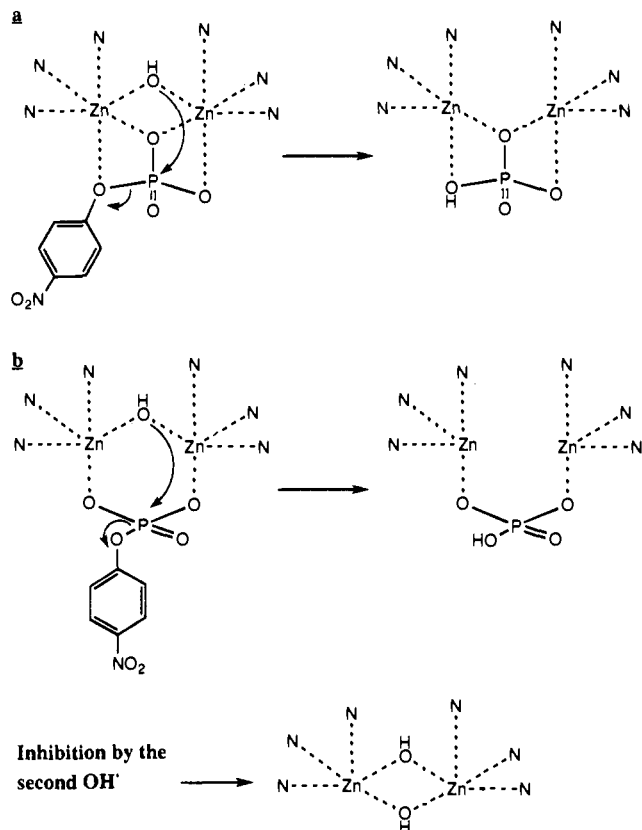
Figure 8. Two alternative mechanisms for the hydrolysis of p -nitrophenyl phosphate ( 2 ) catalyzed by the double Zn(II) complex of ligand 6 . Mechanism a is analogous to that proposed for the action of alkaline phosphatase, based on X-ray structures, 2b while mechanism b is based on the finding 2b that inorganic phosphate binds to the two Zn(II) atoms of alkaline phosphatase using two different oxygen atoms. Both mechanisms can fit our (somewhat flexible) catalyst, from molecular models, and our data. To avoid clutter in the drawings, the charges on the Zn and O atoms are omitted. Also shown is one way in which a second OH - could inhibit the catalysis, by displacing the substrate. Alternative mechanisms for catalysis and inhibition are also possible.
