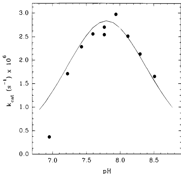
Figure 5. Plot of the rate of hydrolysis of p -nitrophenyl phosphate ( 2 ) ( 2.3 \times 10^{-4} M) catalyzed by the Zn(II) complex of 6 ( 2.3 \times 10^{-4} M) at various pH's in EPPS buffer (10 mM) in water containing 20% DMSO by volume and 50 mM \text{Me}_4\text{N}^+\text{ClO}_4^- . The line is calculated as two titration curves with \text{p}K_1 = \text{p}K_2 = 7.8 .
