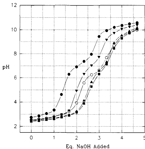
Figure 2. Potentiometric titrations of the ligands alone, as described in the Experimental Section: (●) 1,5,9-triazacyclododecane, (▼) phenylthio ether 11 , (■) 1,3-phenyl dimer 6 , (▲) 1,4-phenyl dimer 7 , (○) 4,4'-biphenyl dimer 9 .
