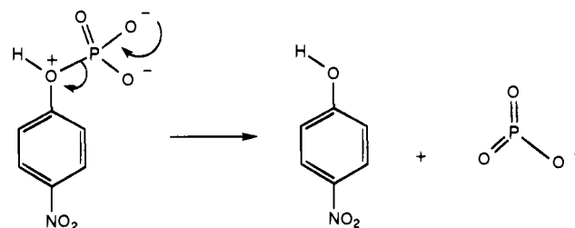
Figure 9. Metaphosphate mechanism for cleavage of p -nitrophenyl phosphate. This mechanism is preferred 12 under normal slightly acidic conditions but is suppressed in favor of the OH - displacement mechanism of Figure 8 by Zn(II) binding to the phosphate.
