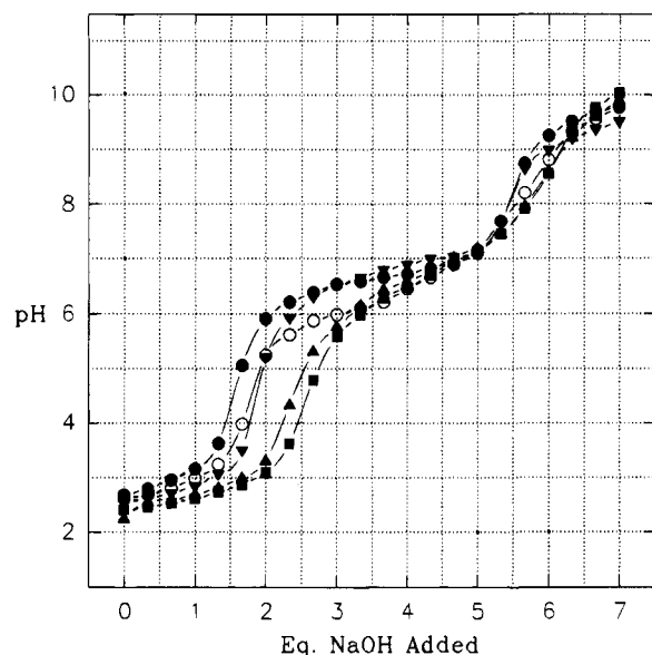
Figure 3. Potentiometric titrations in the presence of 1 equiv of \text{ZnCl}_2 per macrocycle, as described in the Experimental Section: (●) 1,5,9-triazacyclododecane, (▼) phenylthio ether 11 , (■) 1,3-phenyl dimer 6 , (▲) 1,4-phenyl dimer 7 , (○) 4,4'-biphenyl dimer 9 .
