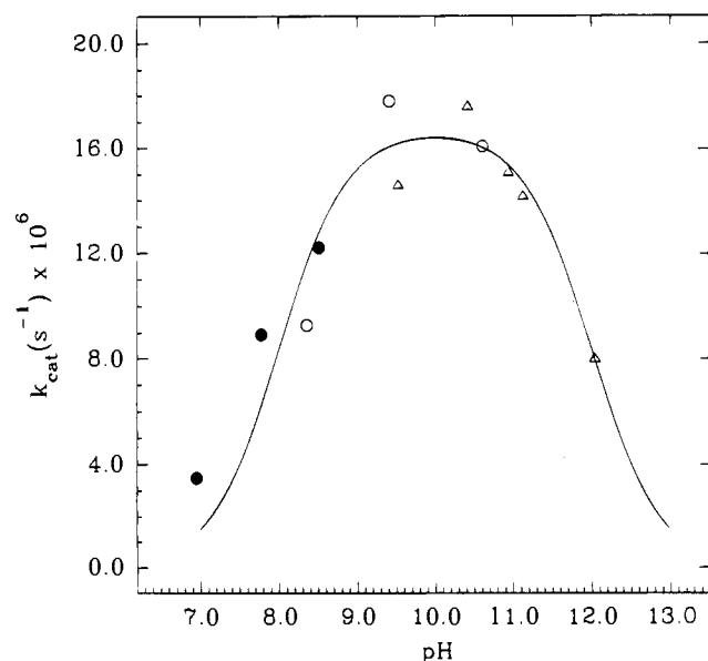
Figure 4. Plot of the rate of hydrolysis of bis( p -nitrophenyl) phosphate ( 3 ) ( 2.3 \times 10^{-4} M) catalyzed by the Zn(II) complex of 9 ( 2.3 \times 10^{-4} M) at various pH's in EPPS (●), CHES (○), and CAPS (△) buffer (10 mM) in water containing 20% DMSO by volume and 50 mM \text{Me}_4\text{N}^+\text{ClO}_4^- . The background rates in the absence of catalyst are subtracted. The line is calculated as two titration curves with \text{p}K_1 = 8 and \text{p}K_2 = 12 .
