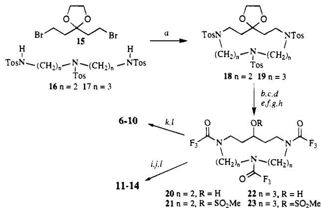
Figure 1. Synthesis of compounds 6–14. (a) Cs 2 CO 3 , DMF, 90–110 °C, 15 h, 45%. (b) HClO 4 , CH 2 Cl 2 , room temperature (RT), 30 min. (c) NaBH 4 , MeOH (from 18 , 83%), EtOH (from 19 , 91%), RT, 15 min. (d) (1) NaH, 2–5 mol % imidazole, THF; reflux, 1 h; (2) MeI, reflux, 3 h. (e) Li/NH 3 , –78 °C to RT, 3 h, 45–82% through steps d and e. (f) Trifluoroacetic anhydride, ( i -Pr) 2 NEt, CH 2 Cl 2 , 0 °C to RT, 30 min, 71–79%. (g) BBr 3 , CH 2 Cl 2 , 0 °C to RT, 20 min, 81%. (h) MesCl, ( i -Pr) 2 NEt, CH 2 Cl 2 , 0 °C, 15 min, 82%. (i) Protected 14 from 22 , Ph 3 P, DIAD, THF, thiophenol, 0 °C to RT, overnight, 43%. (j) Protected 11 (22%) and 12 (46%) from 21 , sodium salt of the appropriate thiol in dimethylimidazolone (DMI), 45 °C, overnight. (k) Protected 6–10 from 21 and 23 , bis-sodium salt of the appropriate dithiol in DMI, 45 °C overnight, 30–70%. (l) NH 3 , MeOH, RT, overnight.
